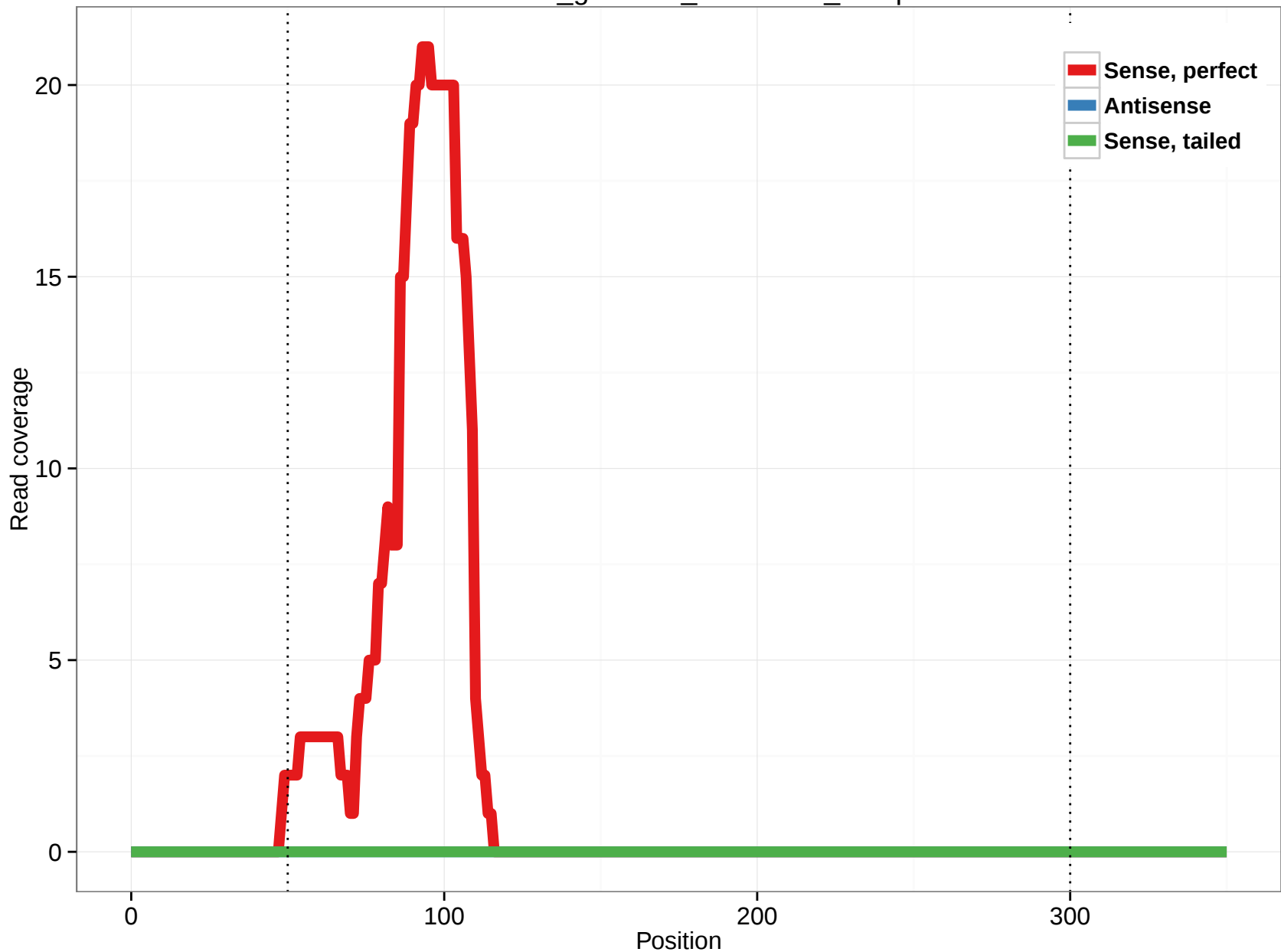
rheMac3_genscan_chr15.137_13.3p
