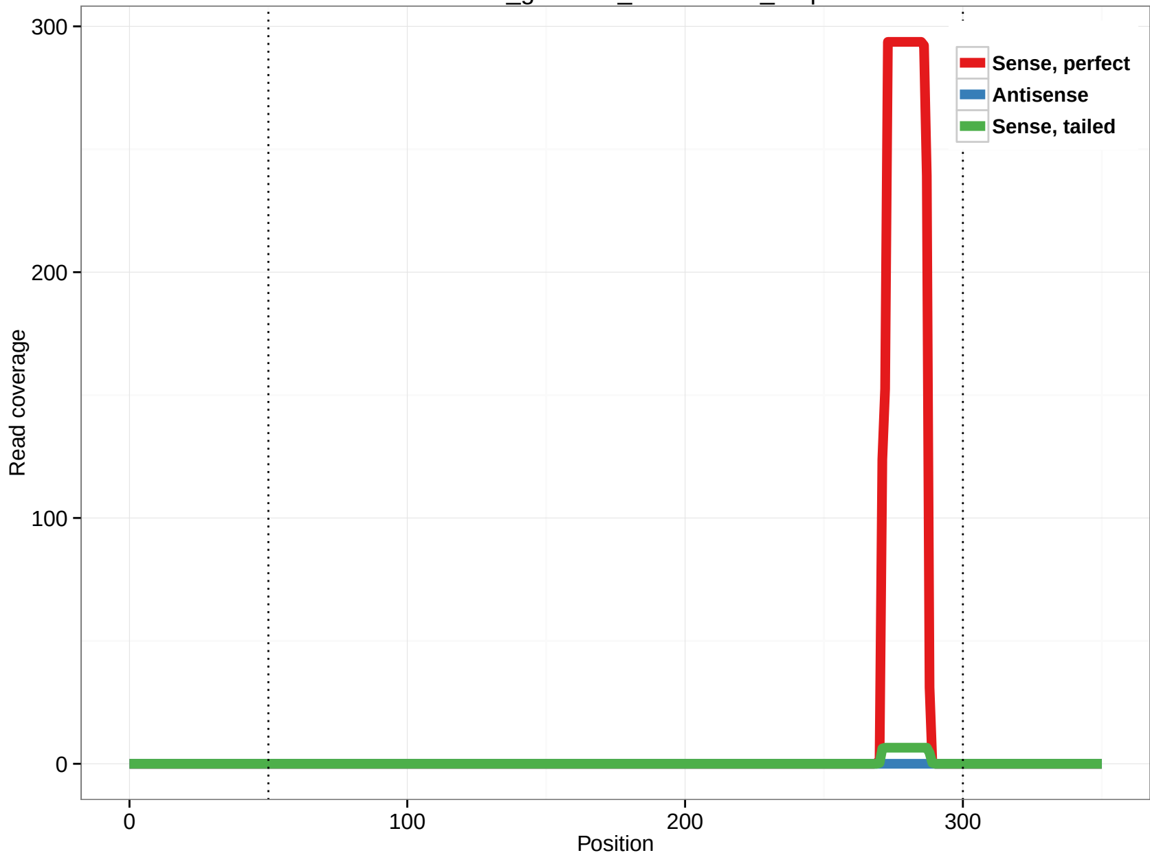
rheMac3_genscan_chr15.1104_1.3p
