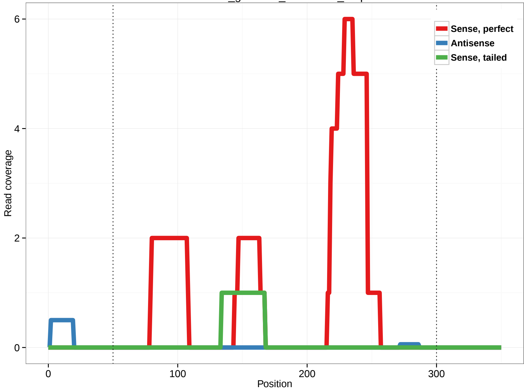
rheMac3_genscan_chr15.102_5.5p
