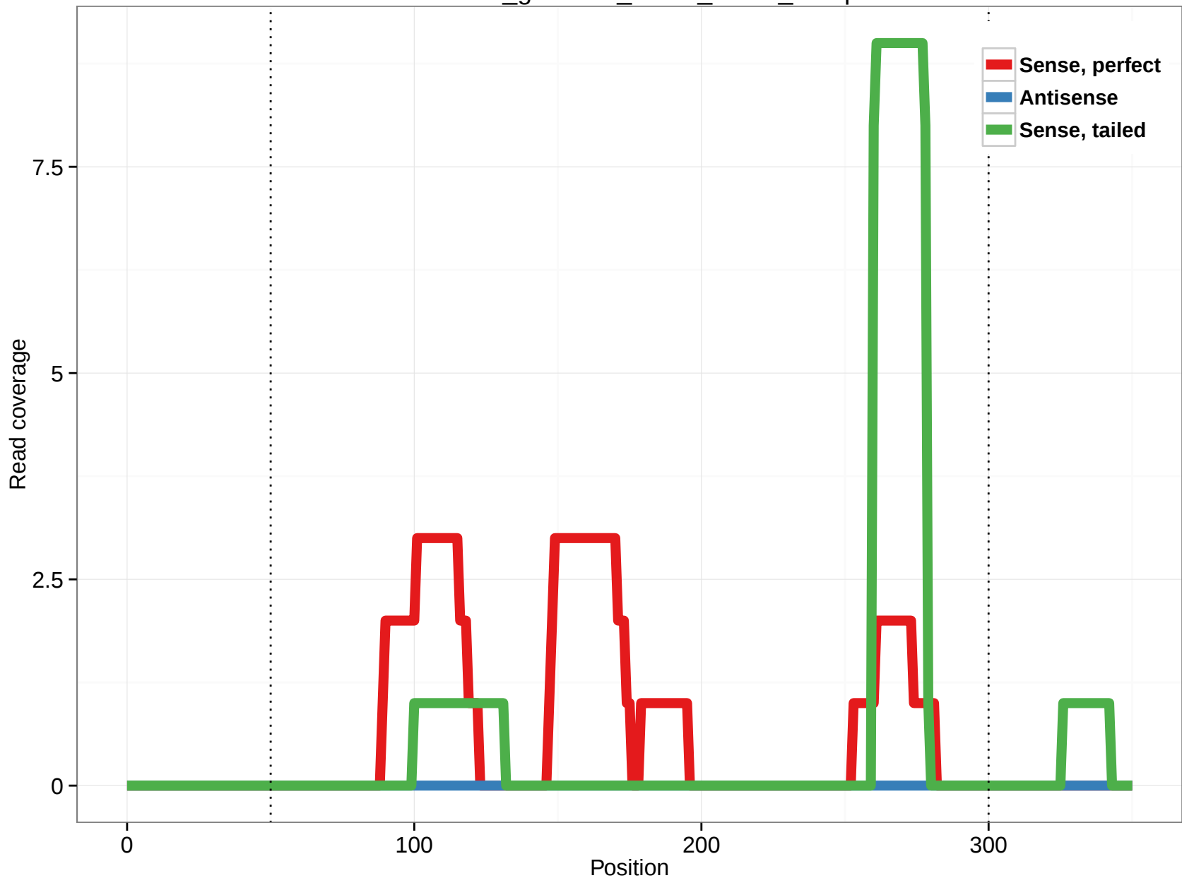
rheMac3_genscan_chr14_77.45_14.5p
