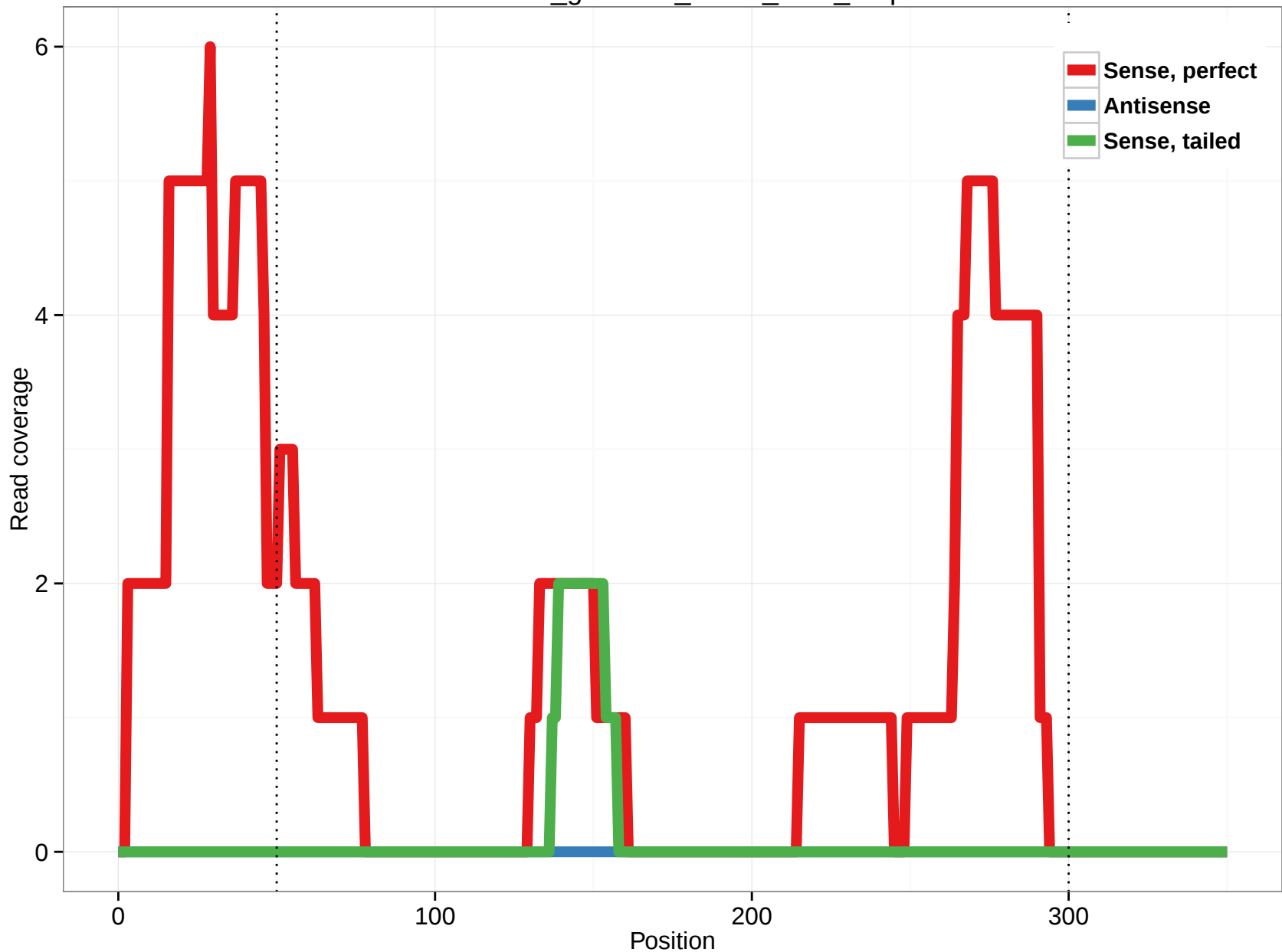
rheMac3_genscan_chr14_76.2_3.5p
