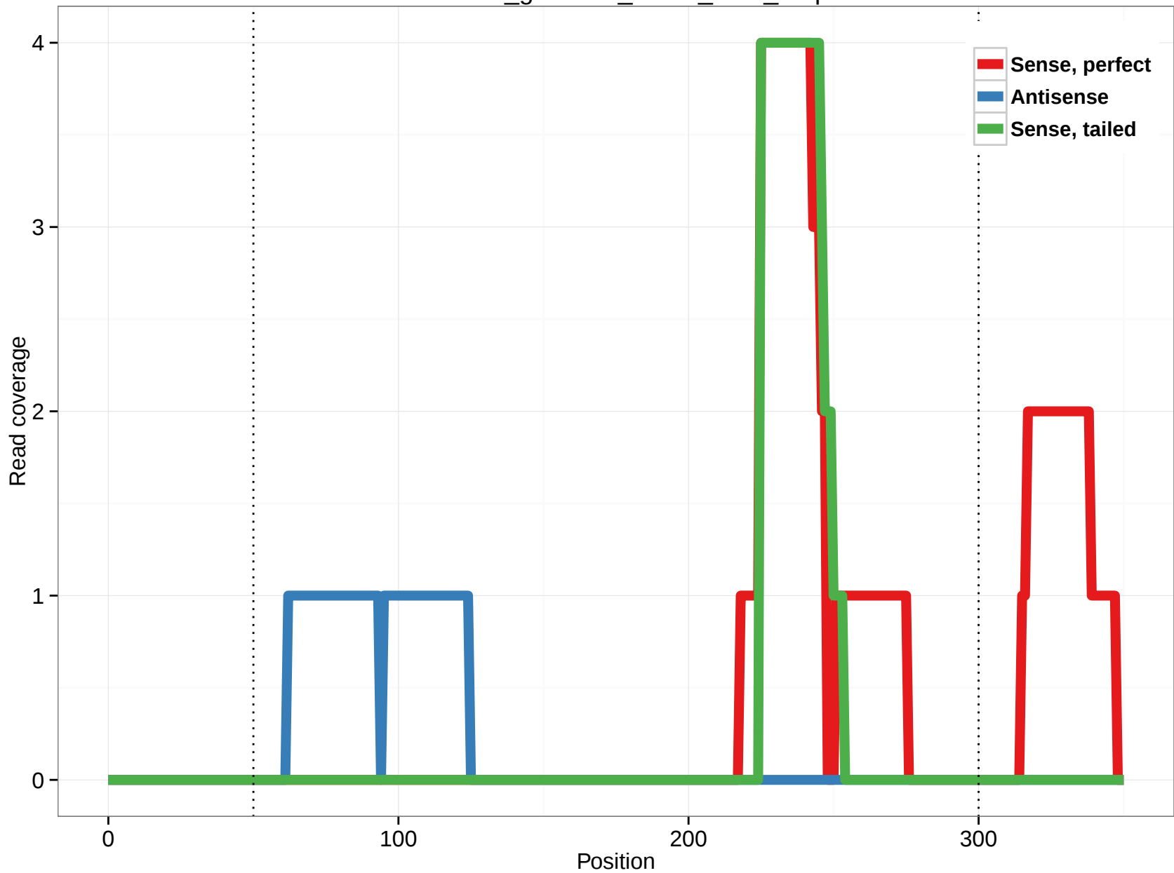
rheMac3_genscan_chr14_75.7_9.3p
