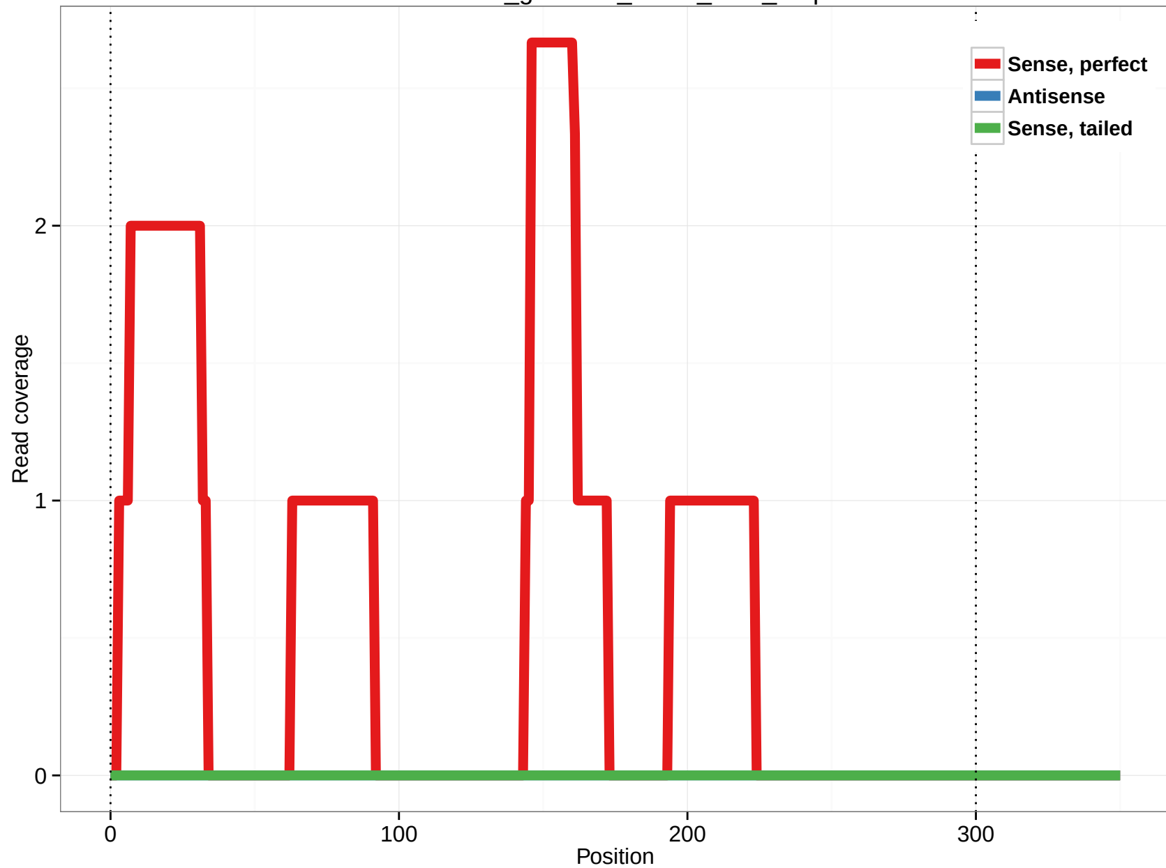
rheMac3_genscan_chr14_75.5_4.3p
