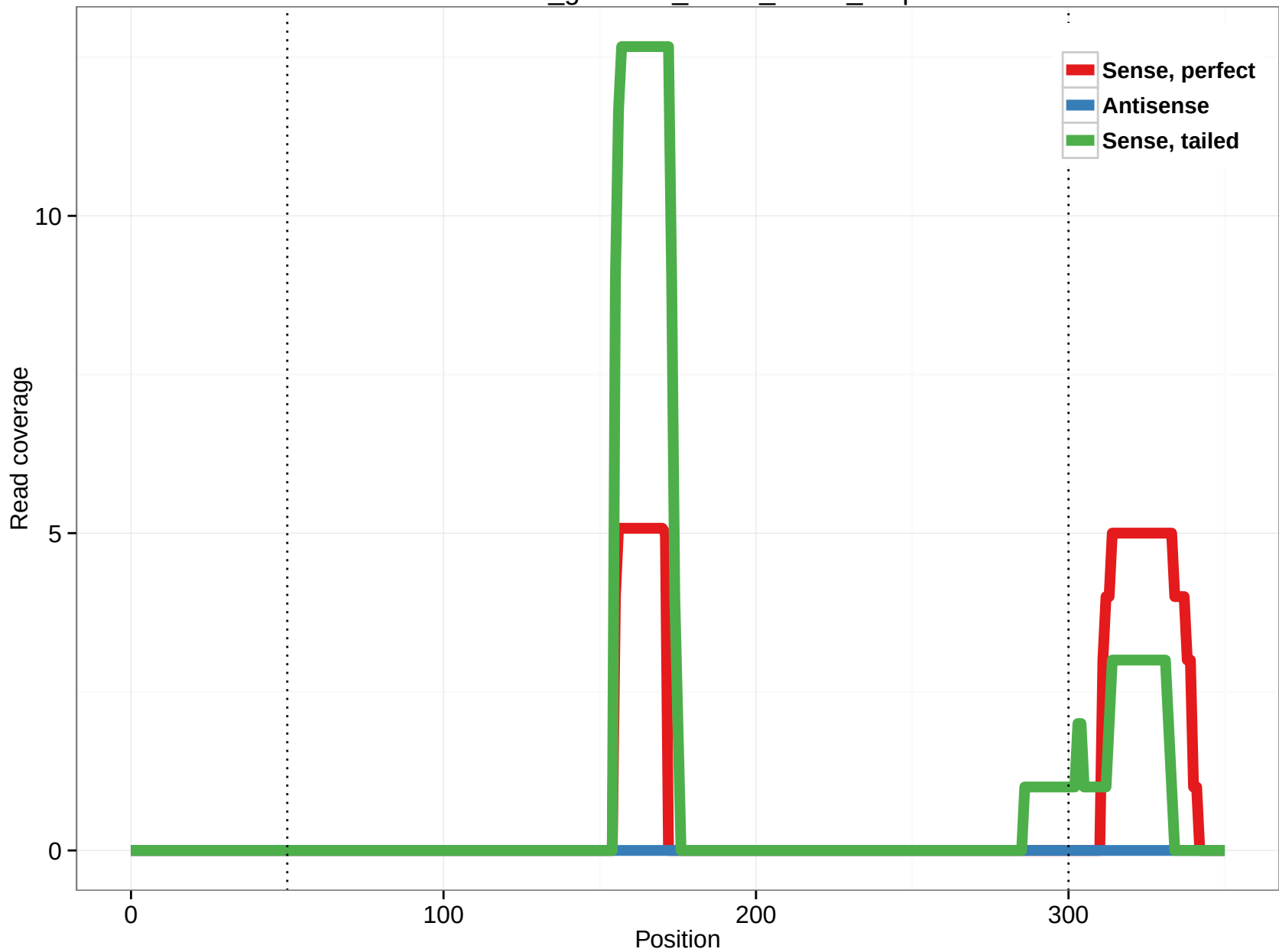
rheMac3_genscan_chr14_75.31_8.3p
