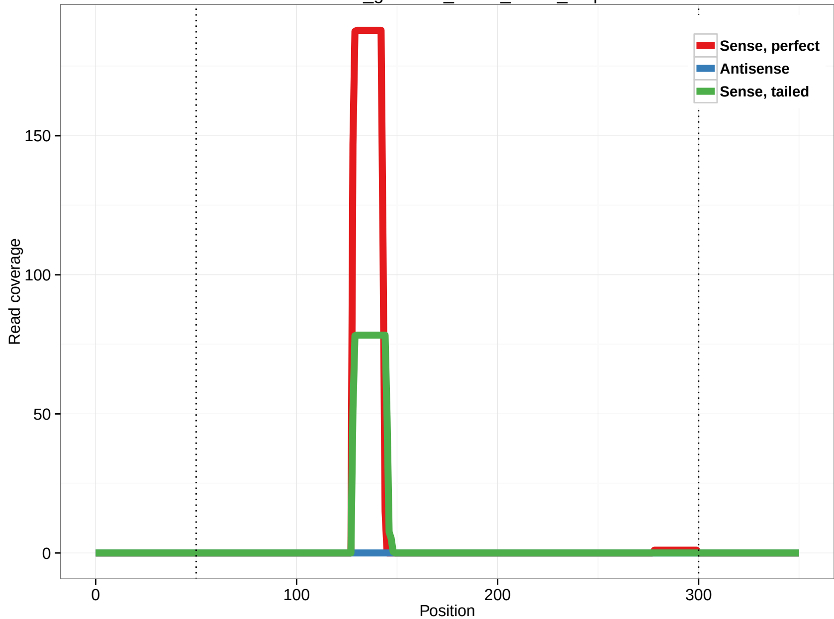
rheMac3_genscan_chr14_75.27_4.3p
