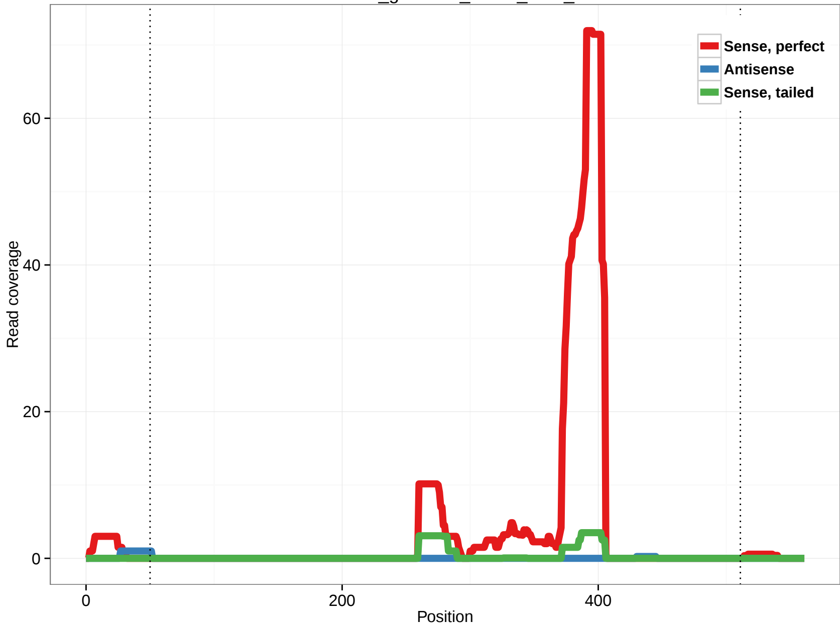
rheMac3_genscan_chr14_75.1_4
