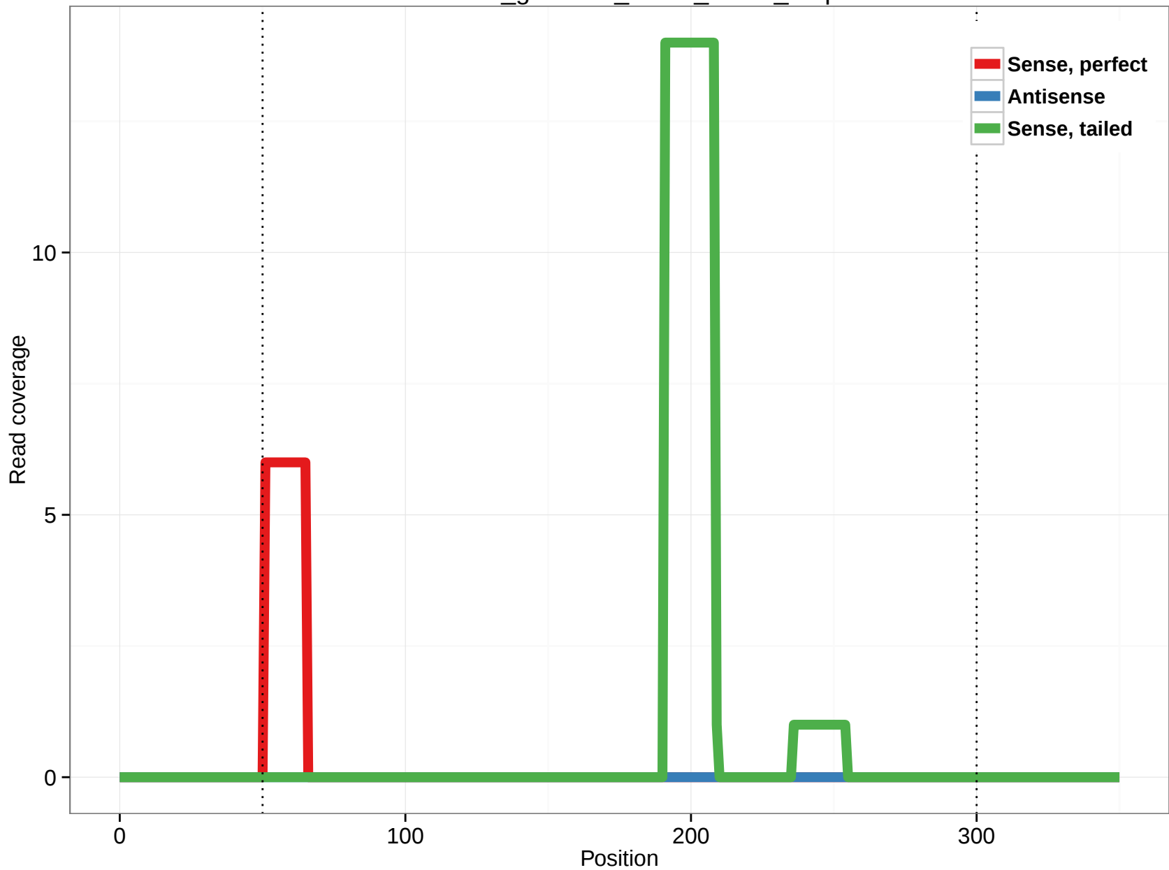
rheMac3_genscan_chr14_75.16_4.3p
