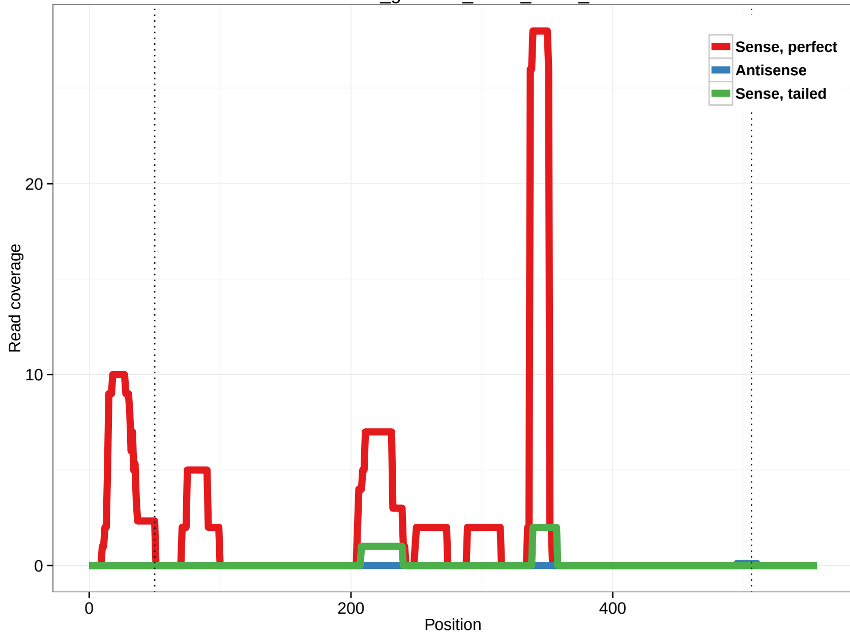
rheMac3_genscan_chr14_75.11_1
