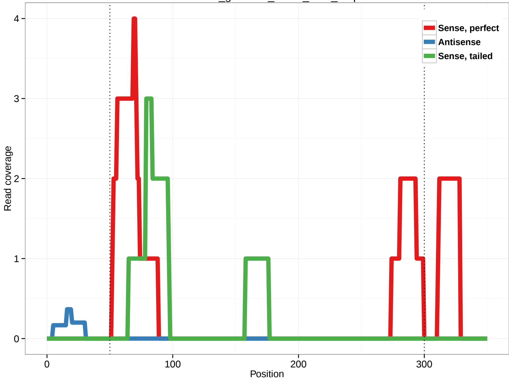
rheMac3_genscan_chr14_72.9_0.5p
