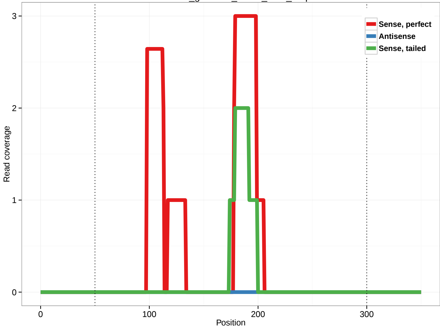
rheMac3_genscan_chr14_72.8_3.5p
