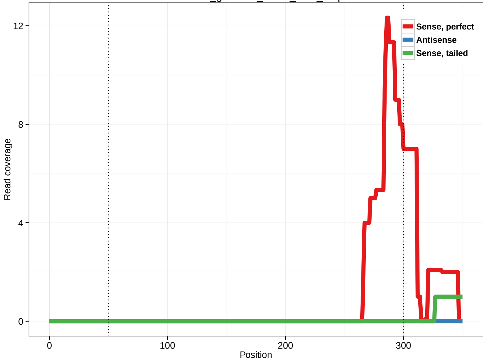
rheMac3_genscan_chr14_72.6_9.5p
