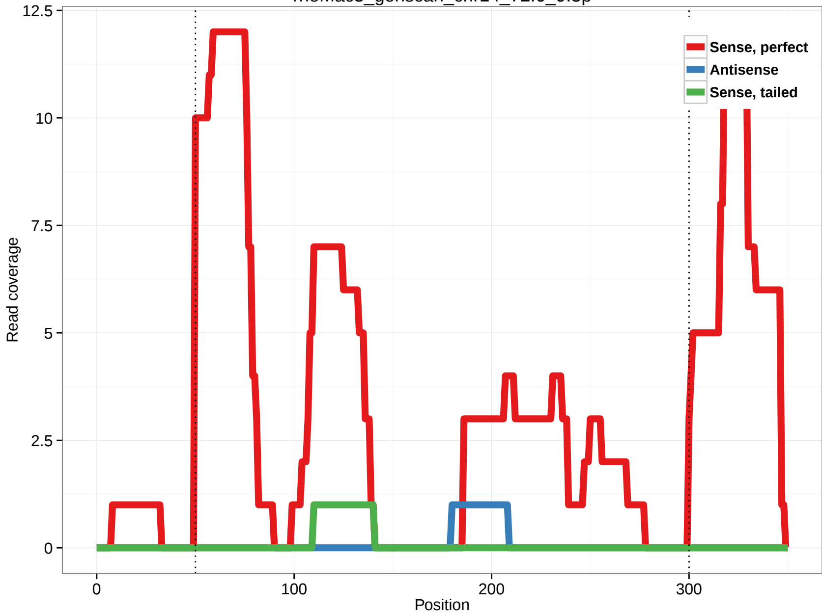
rheMac3_genscan_chr14_72.6_9.3p
