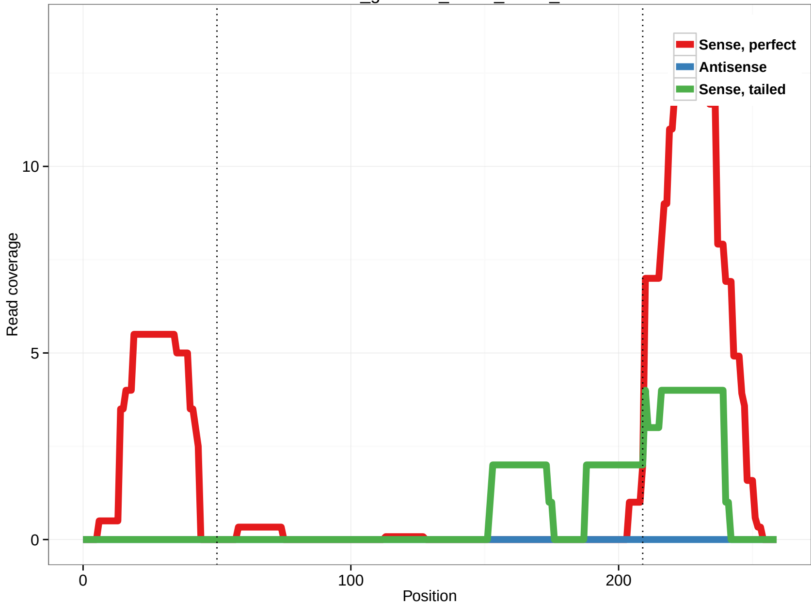
rheMac3_genscan_chr14_70.37_2
