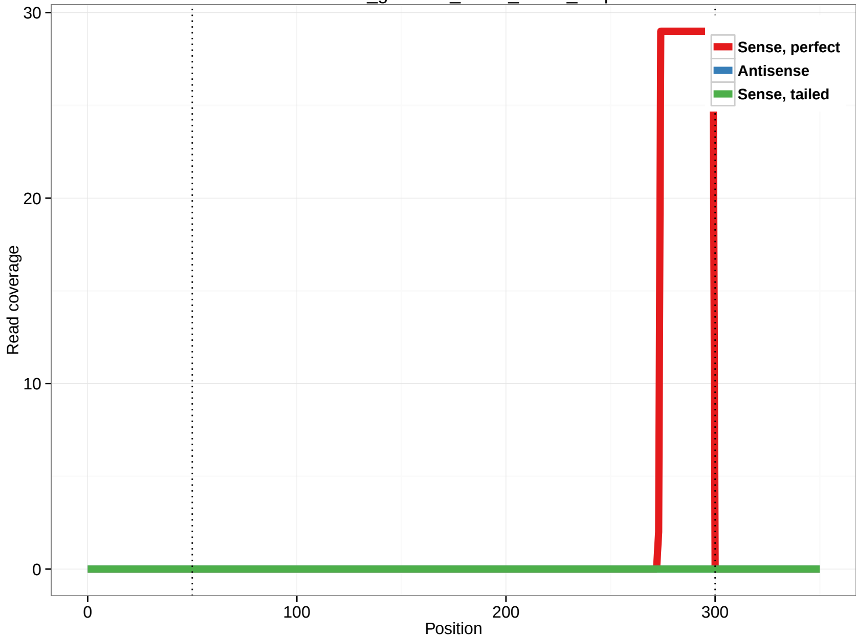
rheMac3_genscan_chr14_70.19_0.3p
