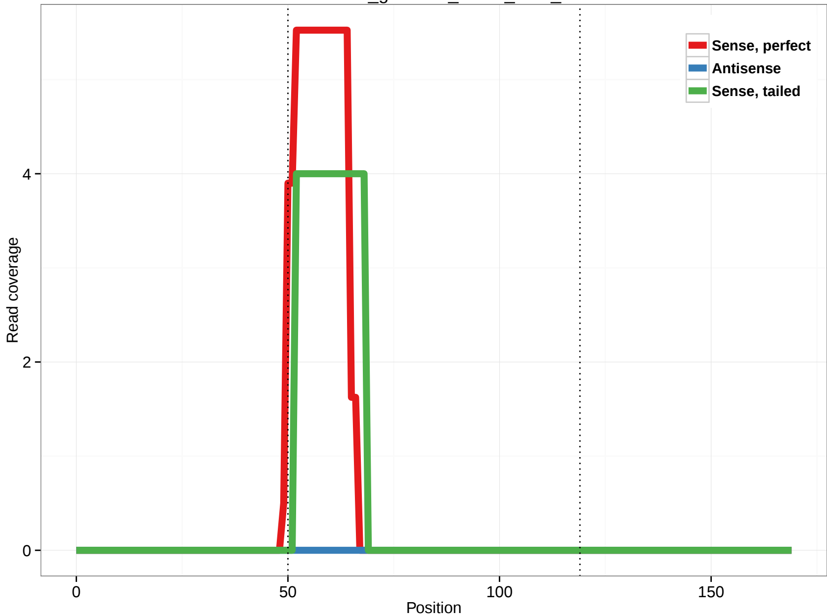
rheMac3_genscan_chr14_68.6_1
