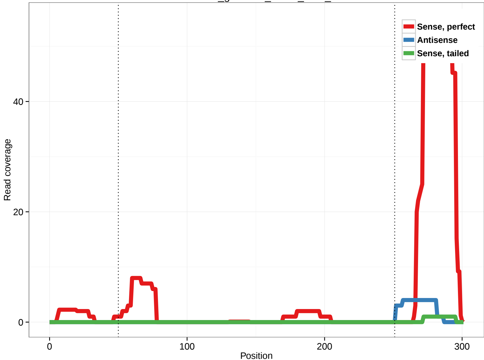
rheMac3_genscan_chr14_55.8_0
