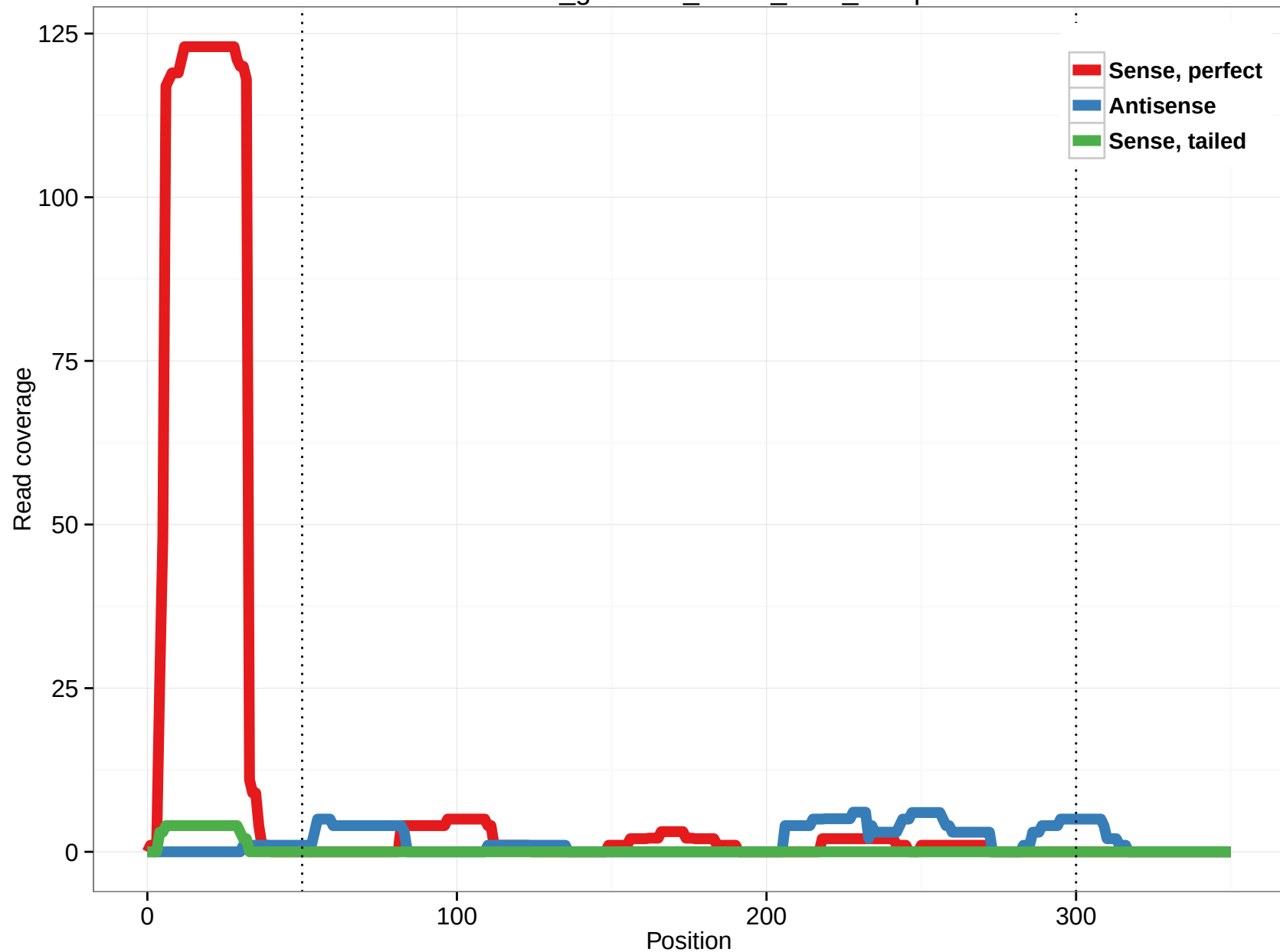
rheMac3_genscan_chr14_51.7_12.5p
