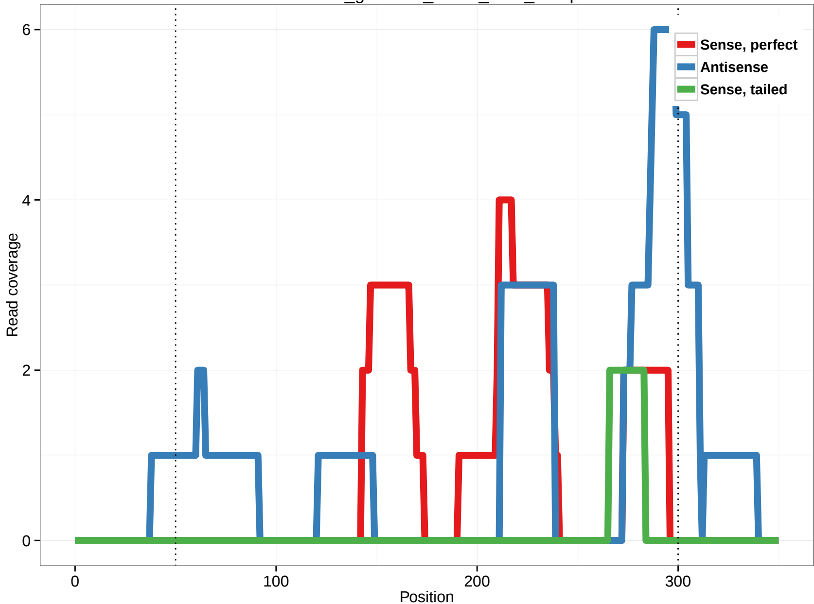
rheMac3_genscan_chr14_51.7_11.3p
