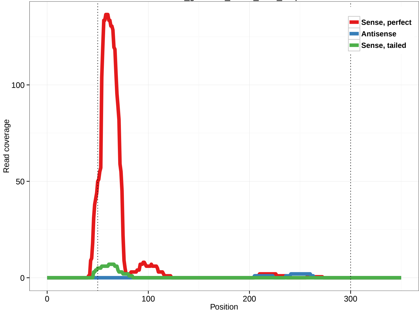
rheMac3_genscan_chr14_48.1_2.5p
