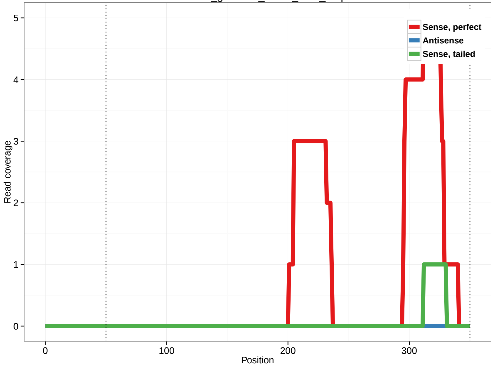
rheMac3_genscan_chr14_44.7_1.5p
