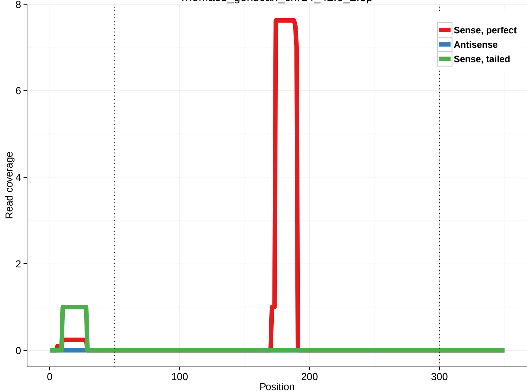
rheMac3_genscan_chr14_42.6_2.3p
