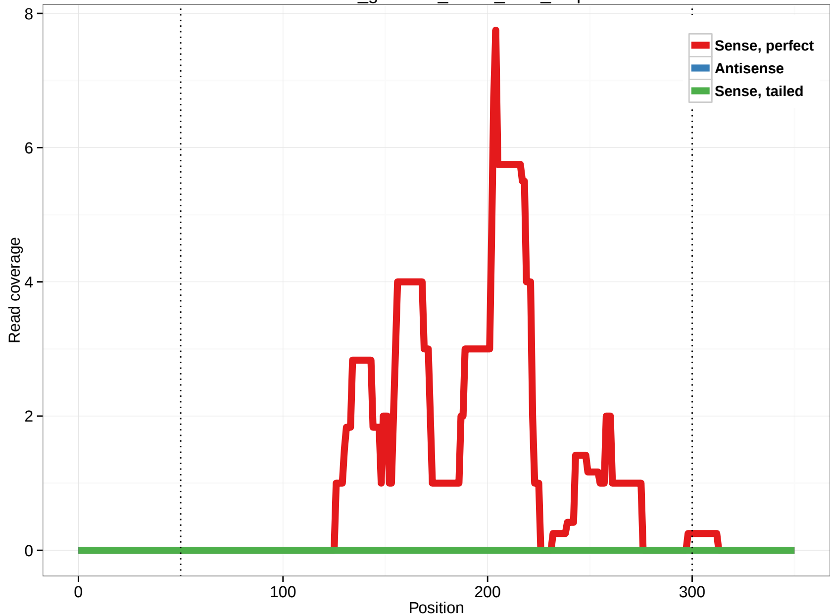
rheMac3_genscan_chr14_42.5_0.5p
