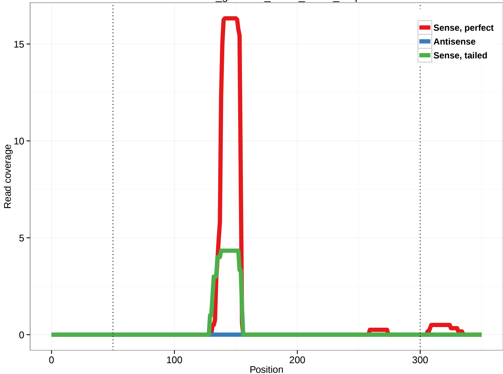
rheMac3_genscan_chr14_42.28_2.3p
