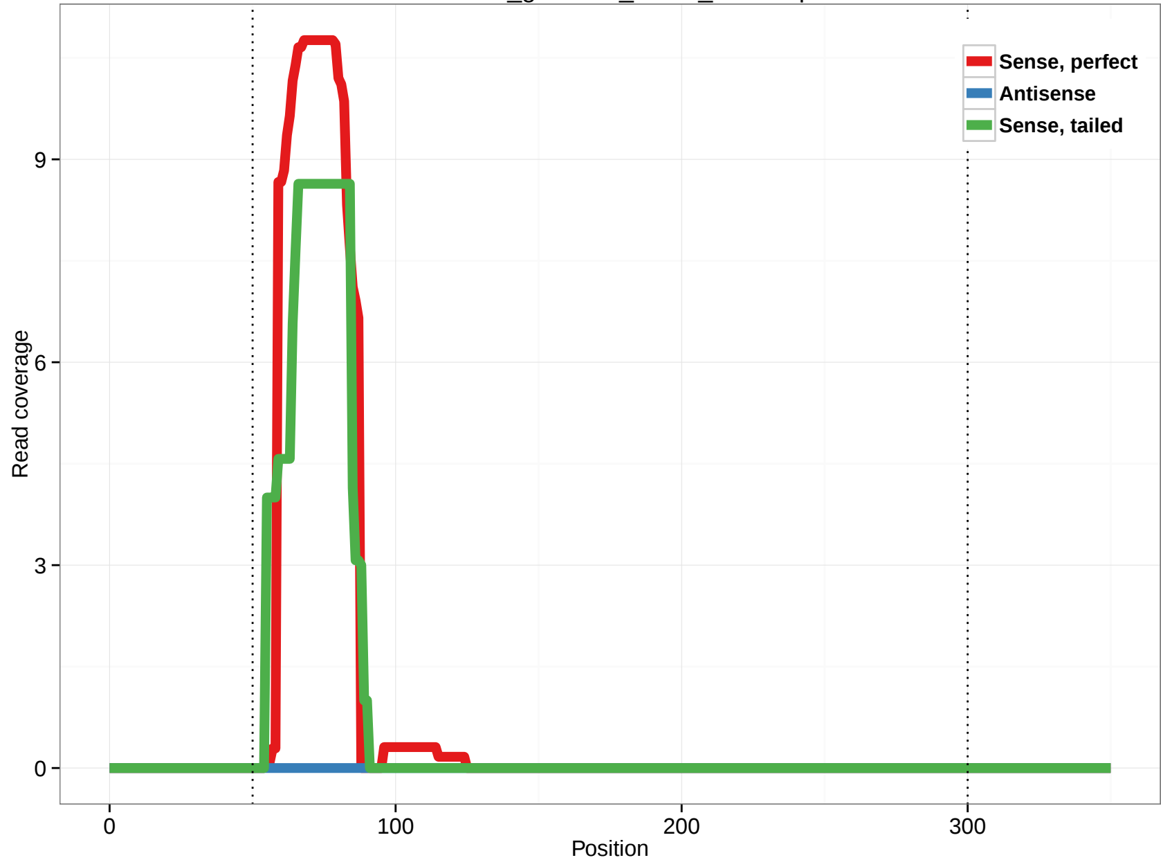
rheMac3_genscan_chr14_42.26.5p
