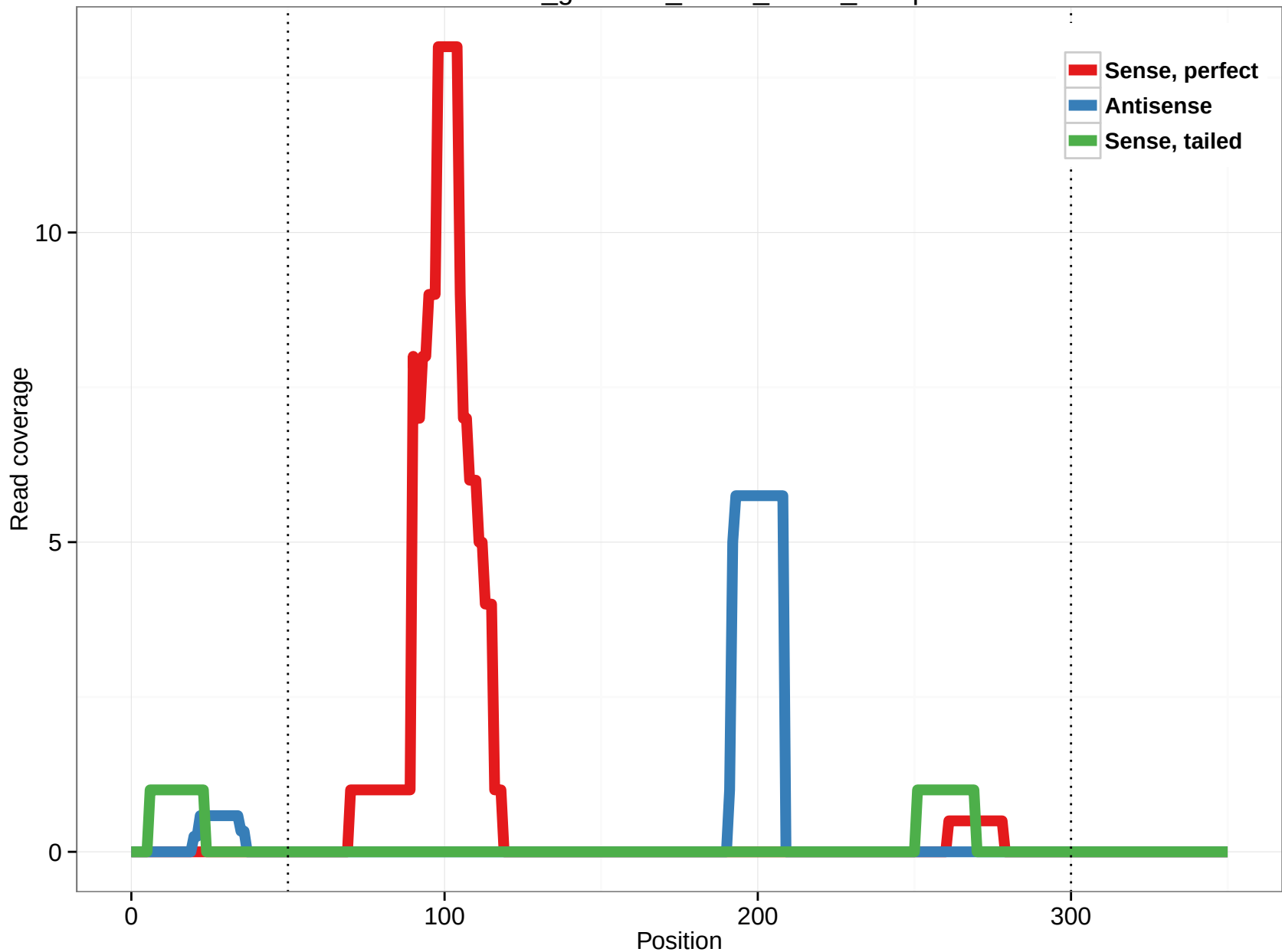
rheMac3_genscan_chr14_42.10_21.5p
