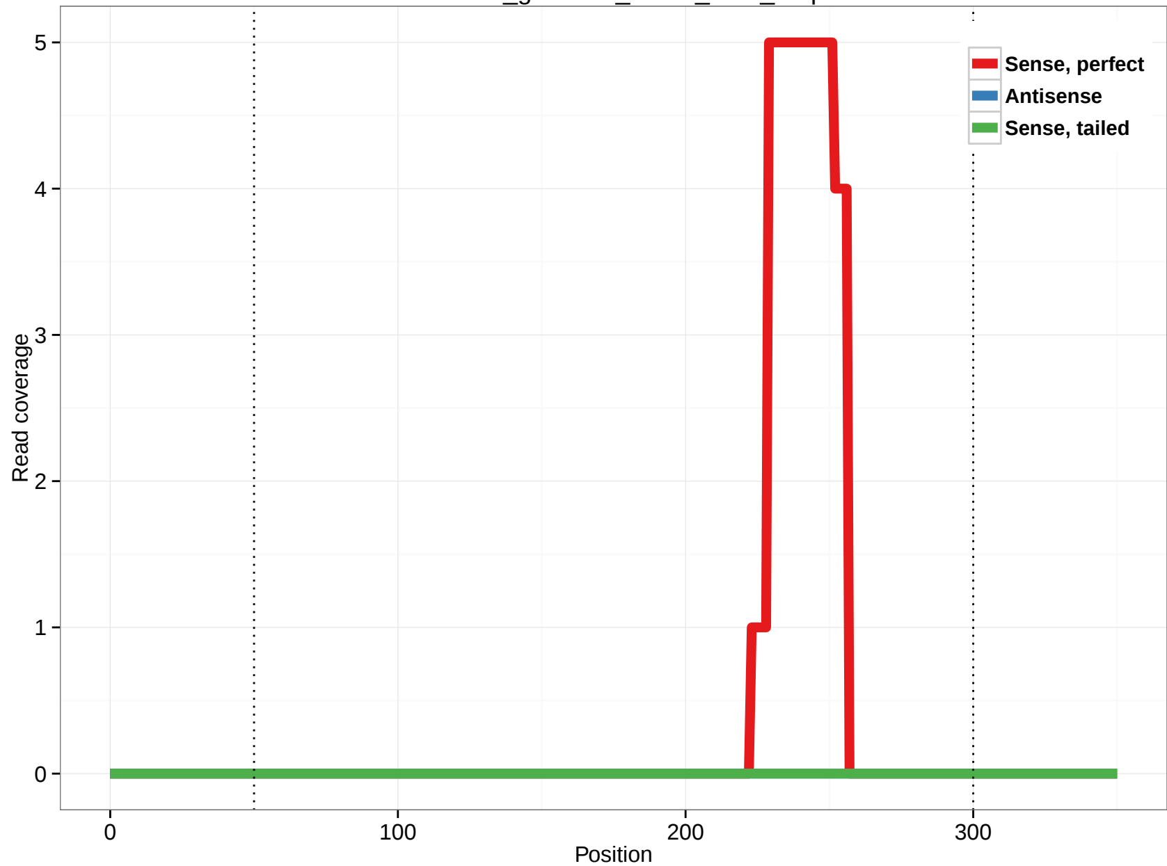
rheMac3_genscan_chr14_30.6_8.5p
