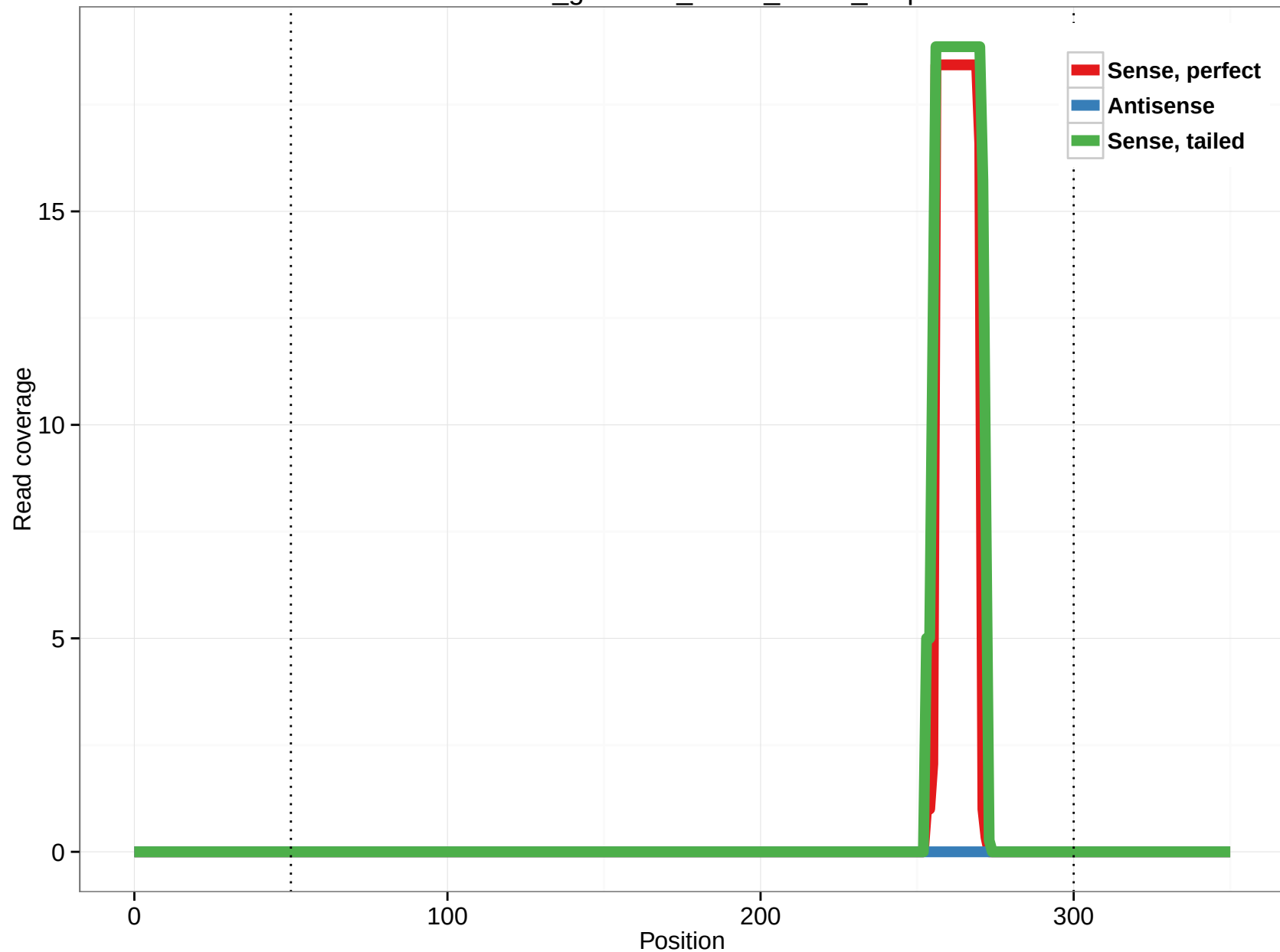
rheMac3_genscan_chr14_29.67_0.5p
