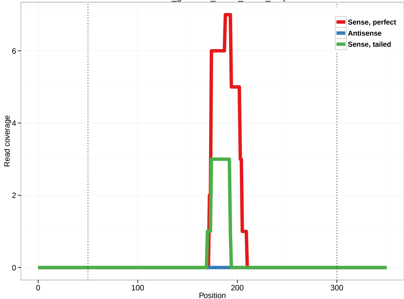
rheMac3_genscan_chr14_29.64_5.3p
