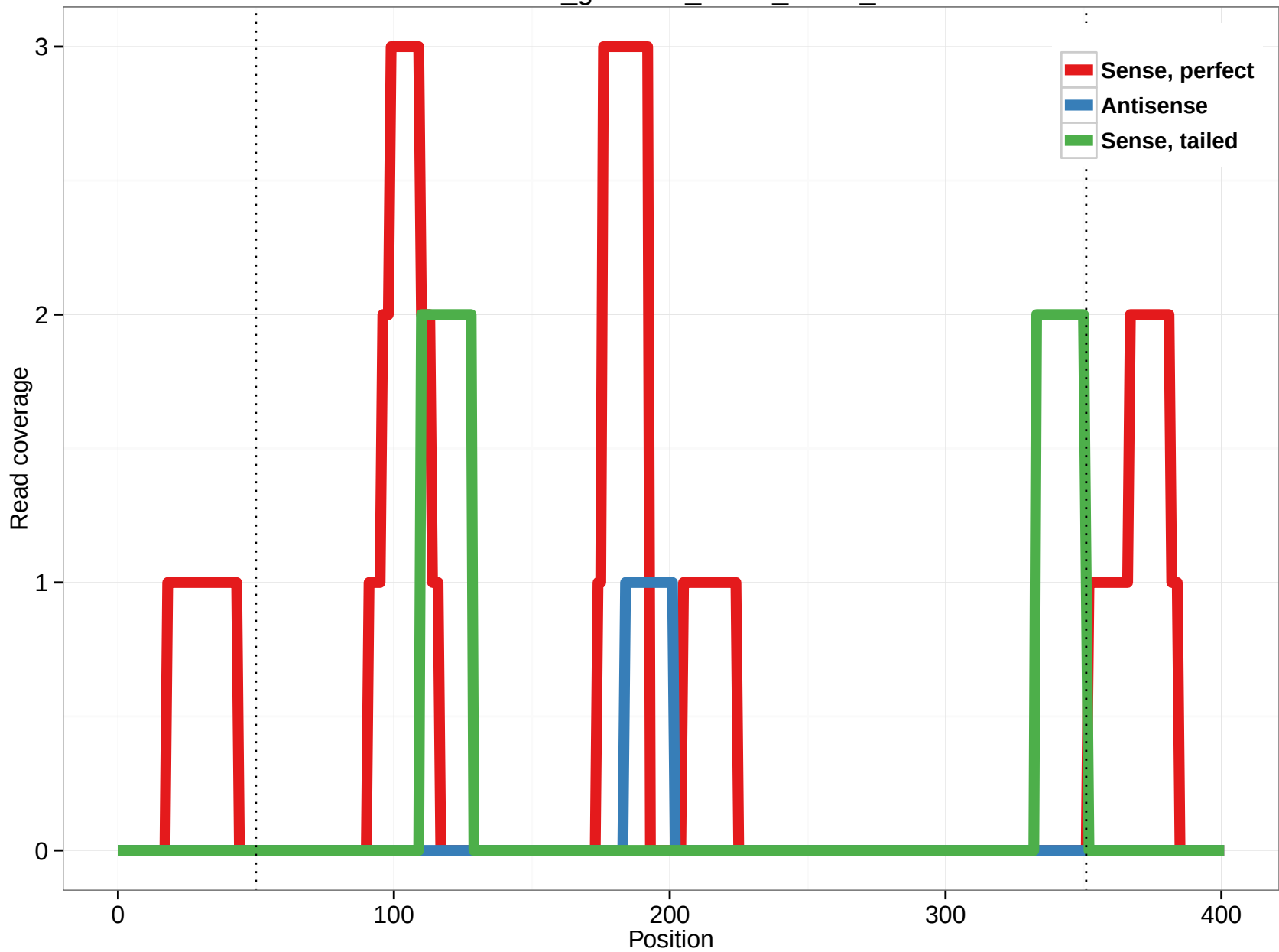
rheMac3_genscan_chr14_29.49_0
