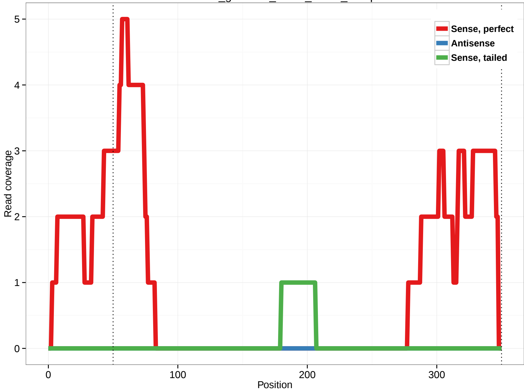
rheMac3_genscan_chr14_29.36_13.5p
