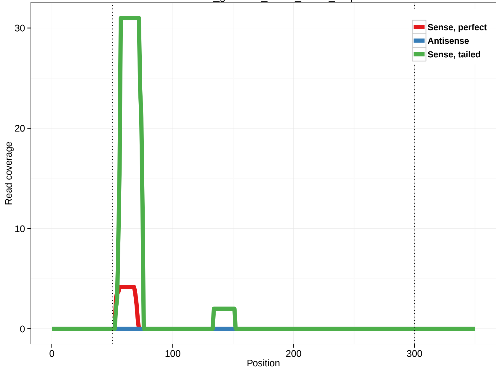
rheMac3_genscan_chr14_29.23_0.5p
