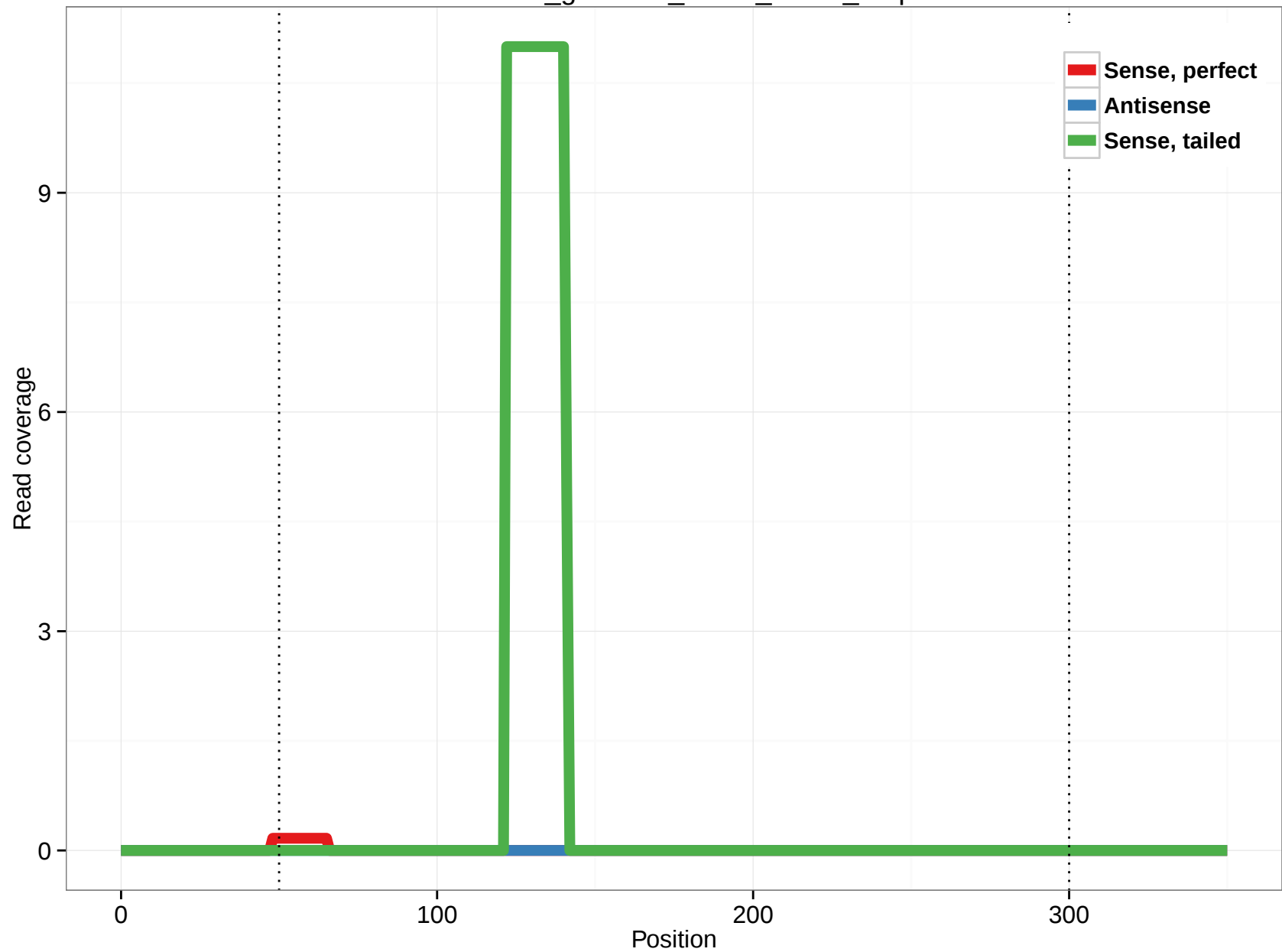
rheMac3_genscan_chr14_24.65_0.5p
