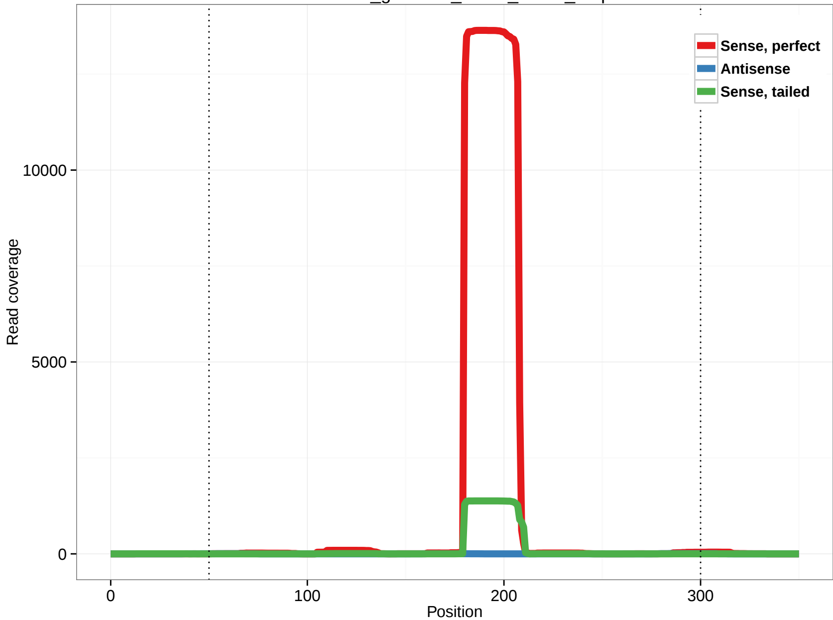
rheMac3_genscan_chr14_24.61_3.5p
