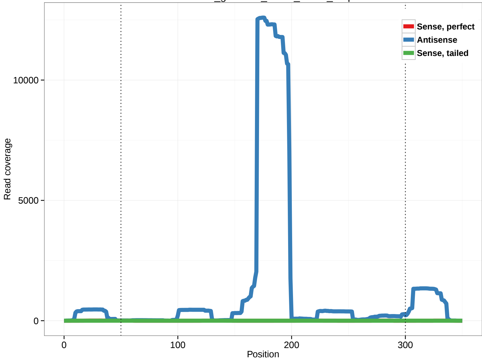
rheMac3_genscan_chr14_24.61_2.5p
