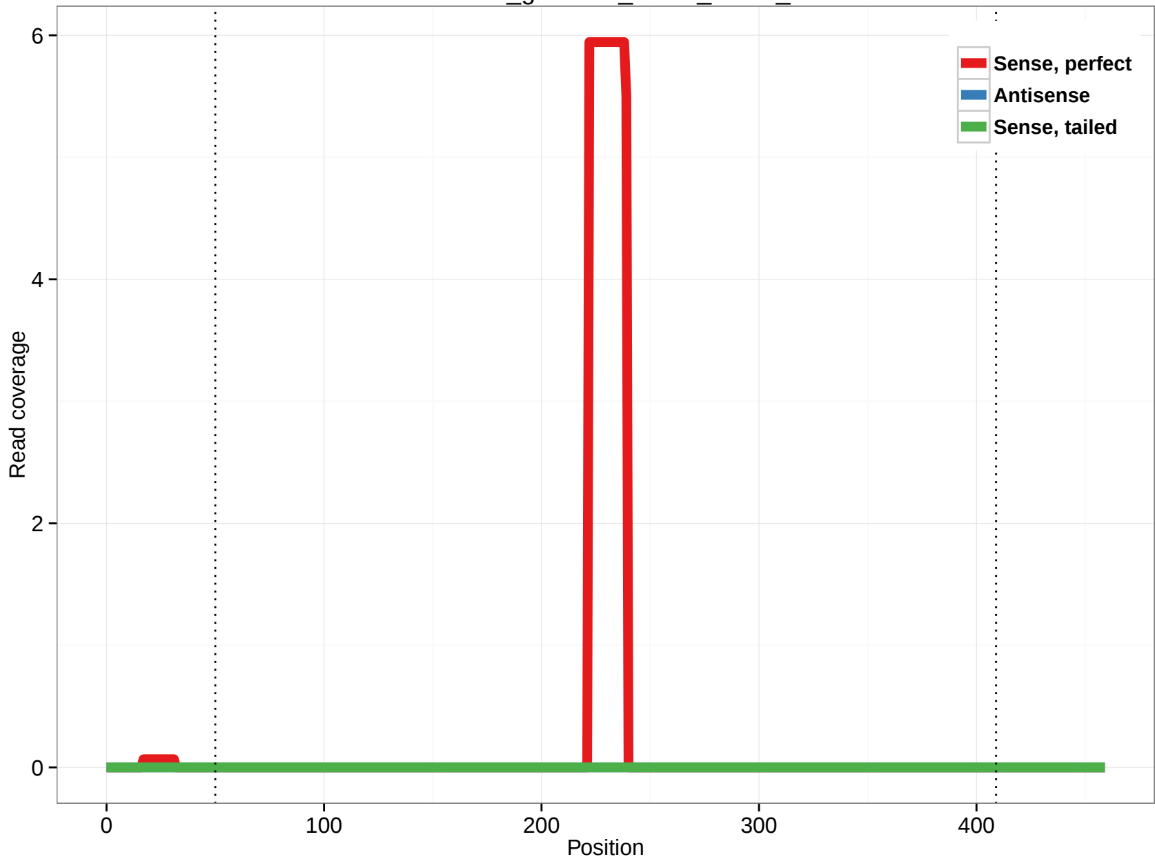
rheMac3_genscan_chr14_24.28_3
