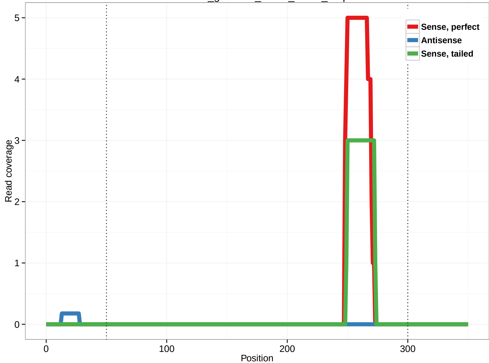
rheMac3_genscan_chr14_24.23_3.3p
