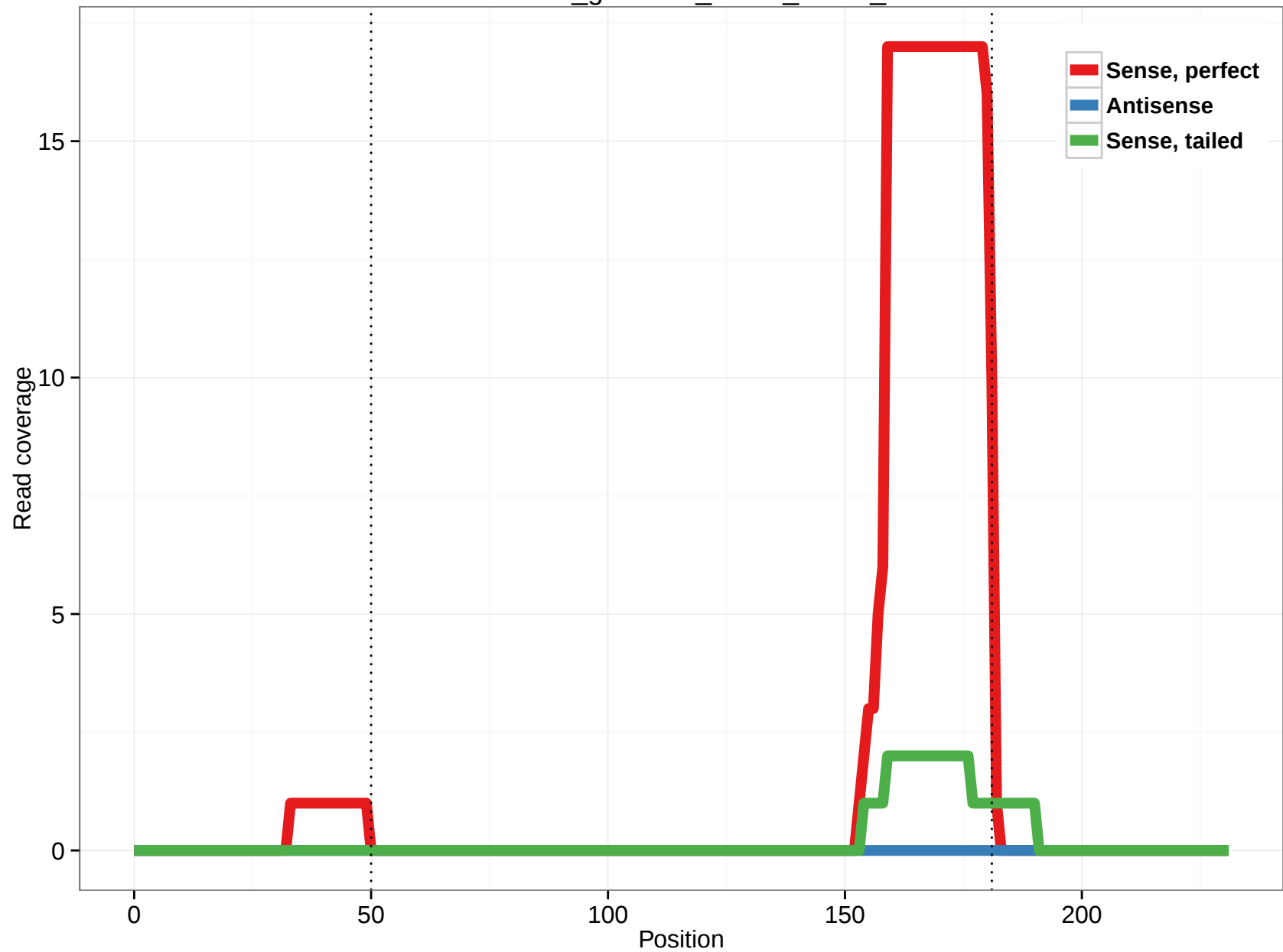
rheMac3_genscan_chr14_16.19_5
