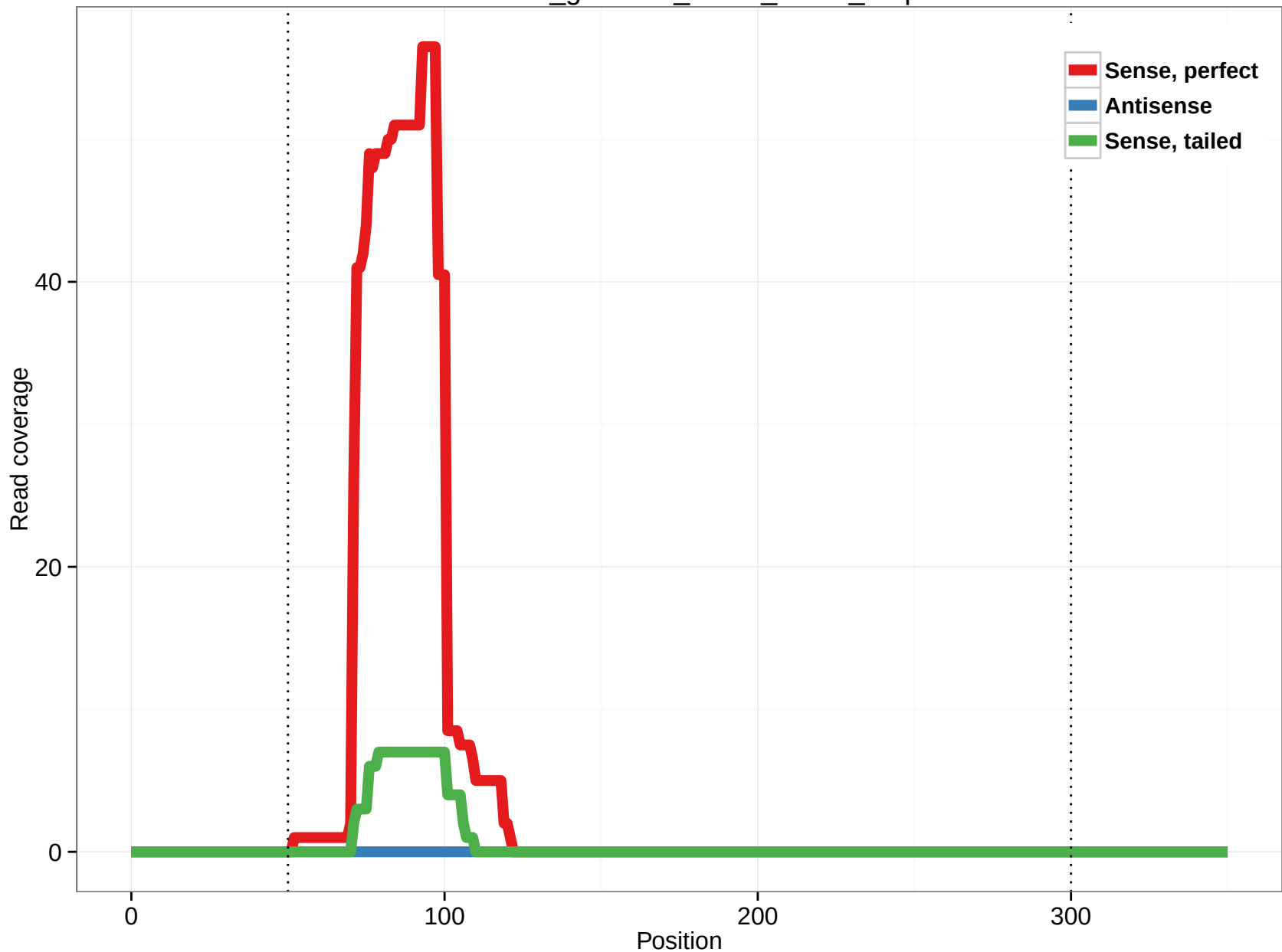
rheMac3_genscan_chr14_16.18_3.3p
