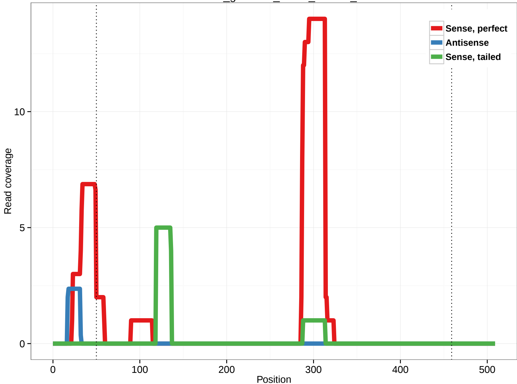
rheMac3_genscan_chr14_126.81_26
