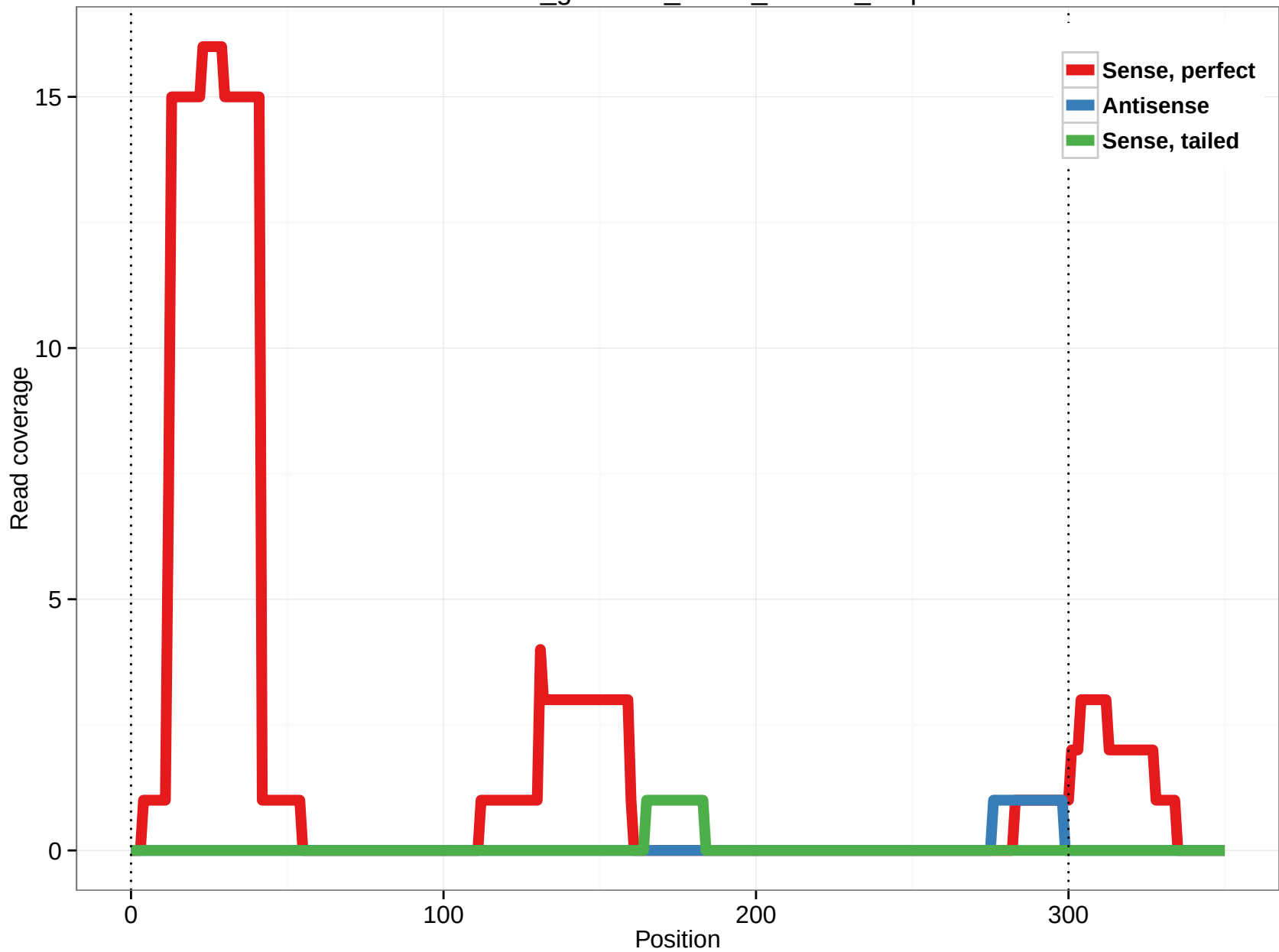
rheMac3_genscan_chr14_126.77_7.3p
