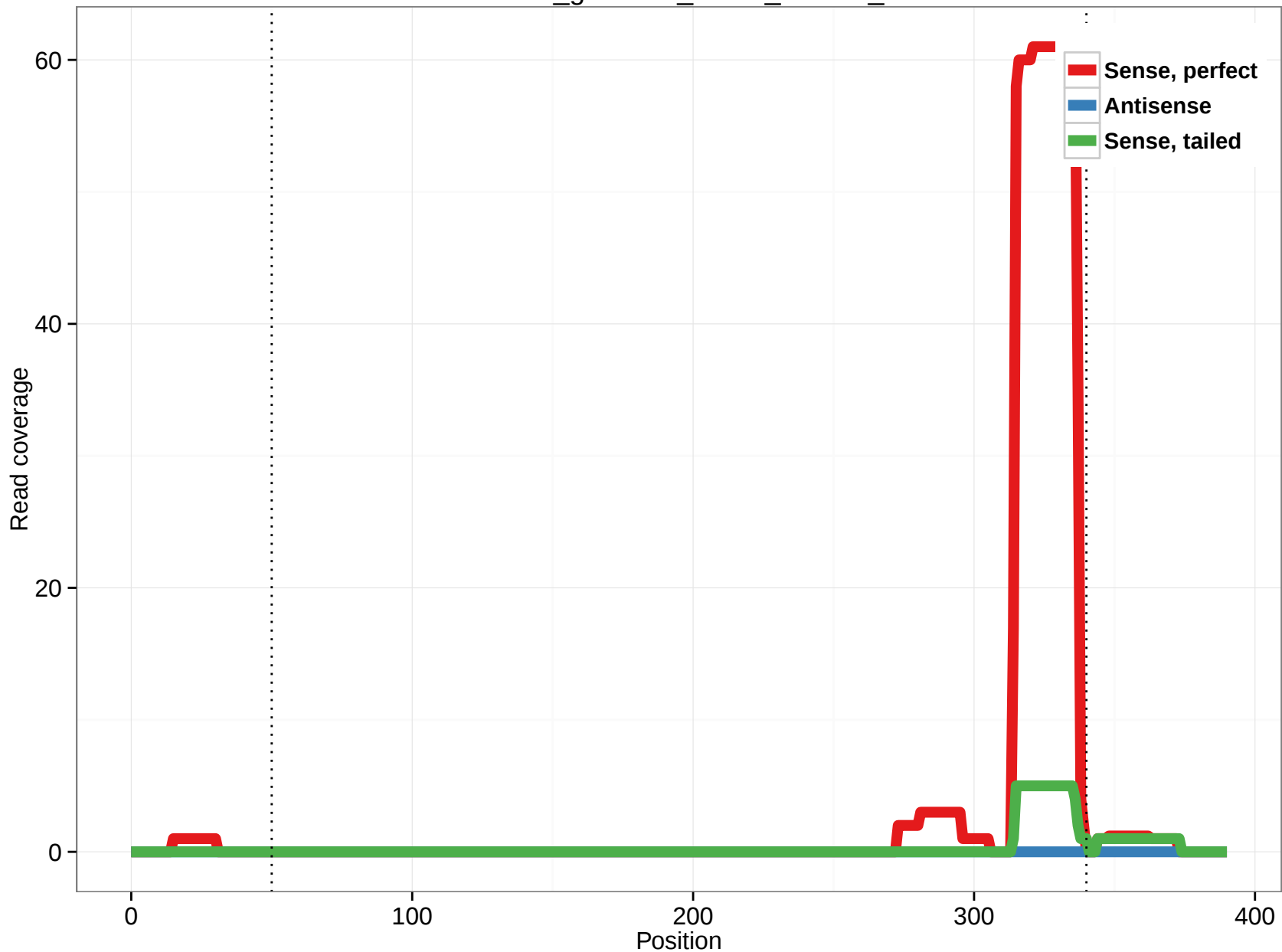
rheMac3_genscan_chr14_126.73_11
