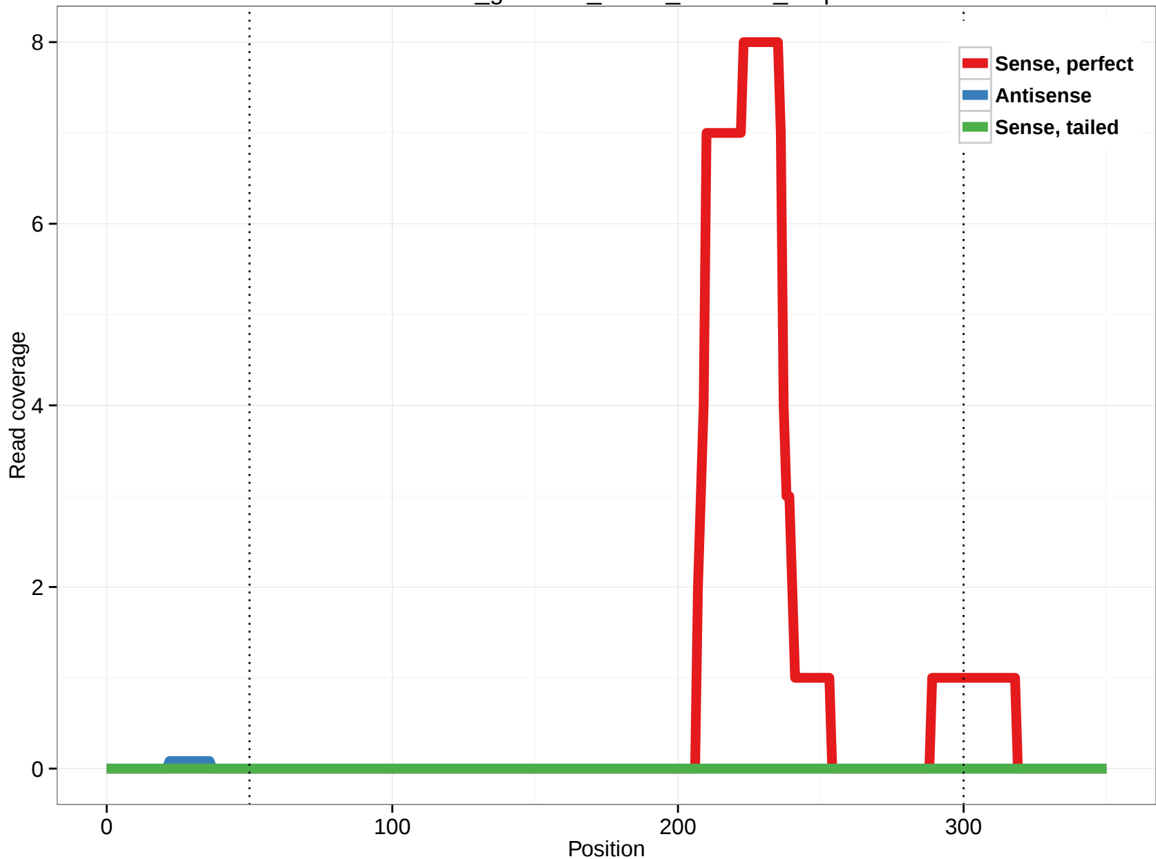
rheMac3_genscan_chr14_126.107_0.5p
