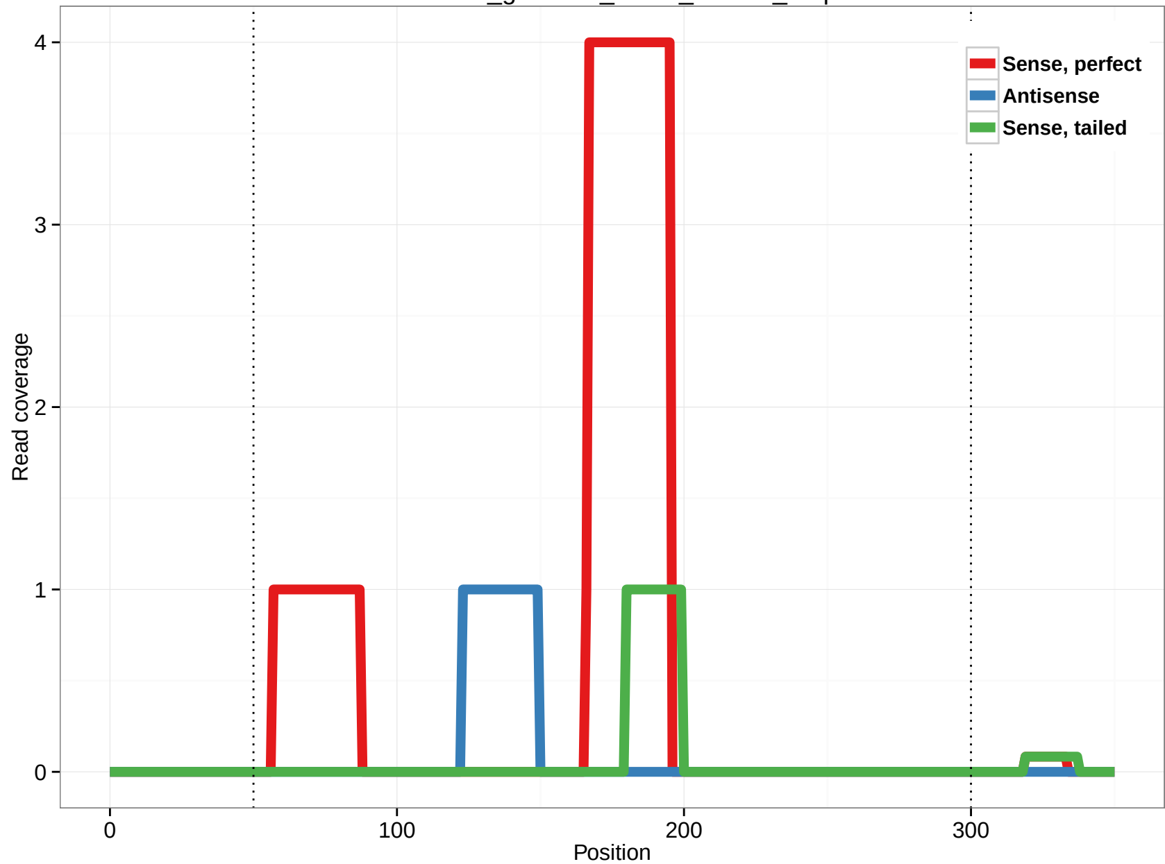
rheMac3_genscan_chr14_124.20_4.5p
