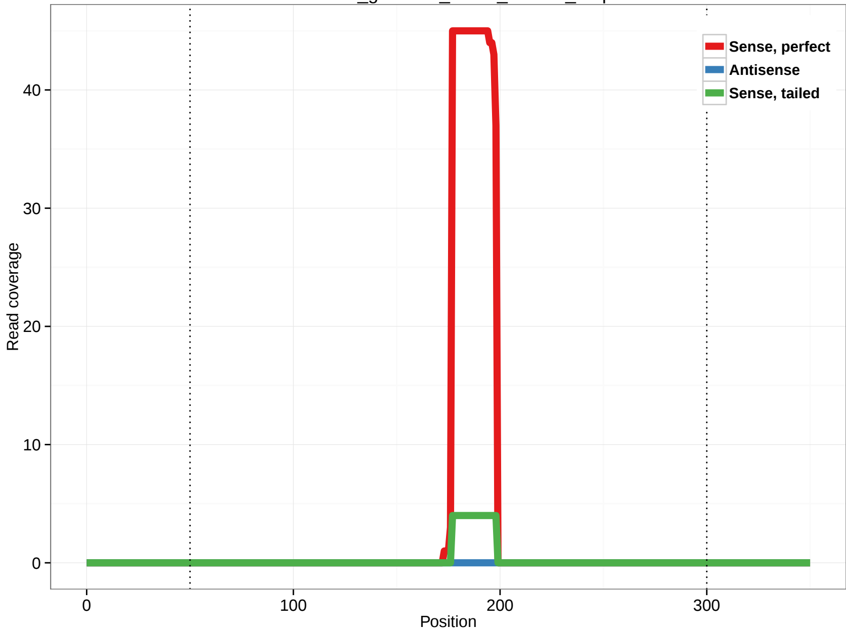
rheMac3_genscan_chr14_122.35_6.3p
