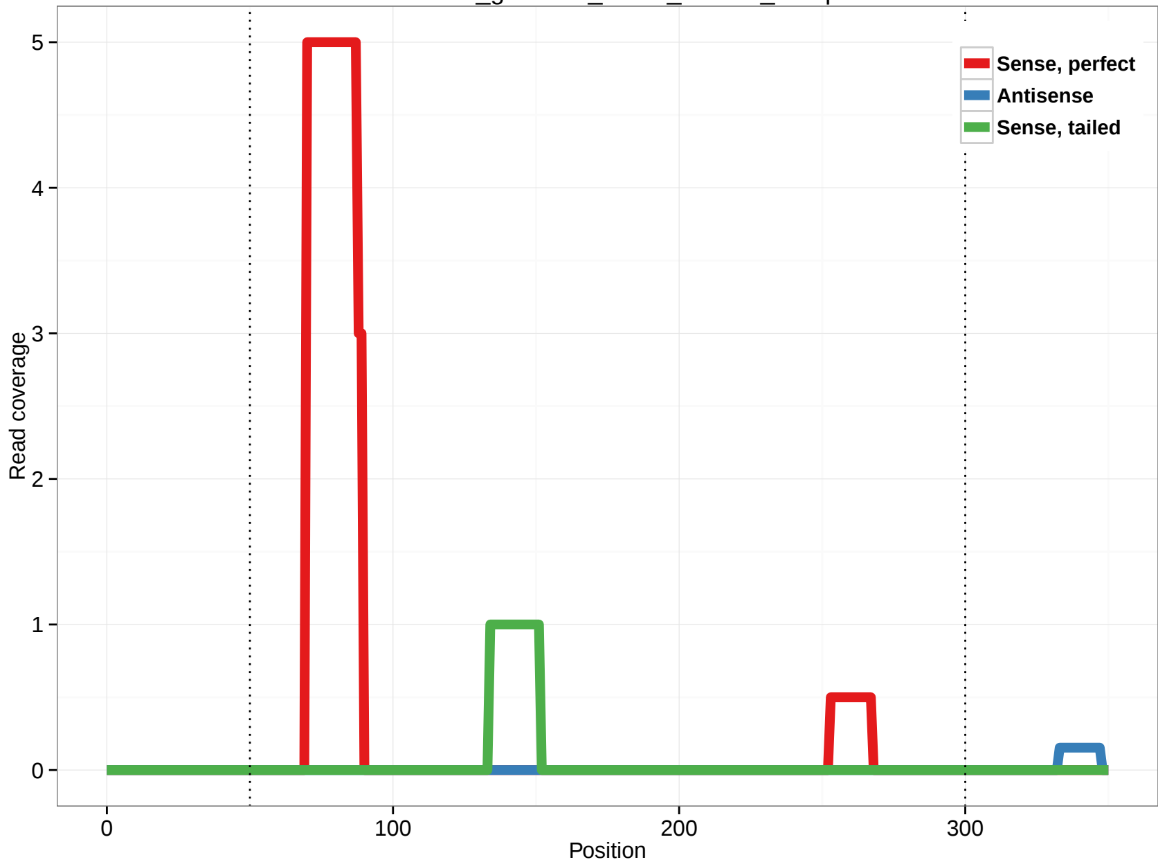
rheMac3_genscan_chr14_122.35_16.5p
