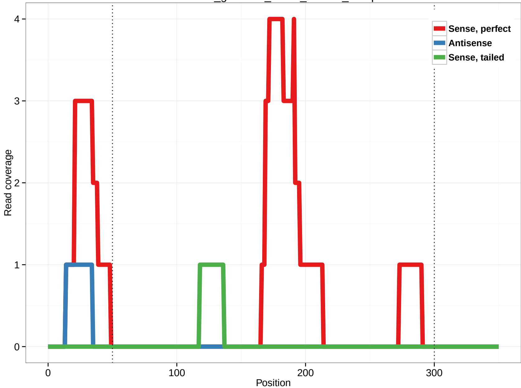
rheMac3_genscan_chr14_119.71_43.5p
